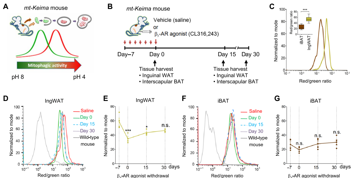
Fig. 1. Regulation of mitophagy during the beige-to-white adipocyte transition. (A) Mitophagic activity in adipose tissues was monitored in vivo by using mitochondrial-targeted Keima ( mt-Keima ) mice. (B) Schematic illustration of the experiments. mt-Keima mice were treated with the \beta_3 -adrenergic receptor ( \beta_3 -AR) agonist CL316,243 or vehicle (saline) for seven consecutive days and harvested at days 0, 15, and 30 after \beta_3 -AR agonist withdrawal. Mitophagic activity in the adipose tissue from each mouse was measured by flow cytometry. (C) Mature adipocytes were isolated from the interscapular brown adipose tissue (iBAT; brown) or the inguinal white adipose tissue (IngWAT; beige) of mt-Keima mice. Signals from green (458 nm) and red (561 nm) channels were detected by flow cytometry. *** P < 0.001 by unpaired Student's t test. n = 8 mice per group. The inset graph shows medians with interquartile range. (D) Mitophagic activity in the IngWAT of mt-Keima mice in (B) based on the ratio of red/green fluorescence intensity. Y axis represents the number of adipocytes normalized to mode. Data are representative of four independent experiments. (E) Quantification of flow cytometry data in (D) by analyzing the median of red/green fluorescence intensity ratio. * P < 0.05 and *** P < 0.001 by one-way analysis of variance (ANOVA) with post hoc test by Tukey's method. n.s., not significant. Data are mean \pm SEM, relative to vehicle-treated mt-Keima mice. (F) Mitophagic activity in the iBAT of mt-Keima mice in (B). Data are representative of four independent experiments. (G) Quantification of flow cytometry data in (F) by analyzing the median of red/green fluorescence intensity ratio. Data are as mean \pm SEM, relative to vehicle-treated mt-Keima mice.
