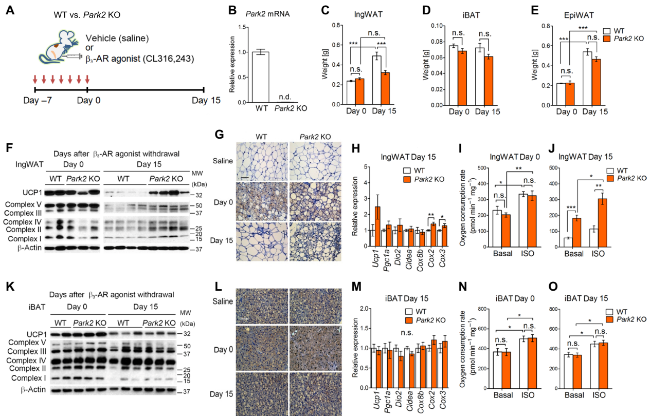
Fig. 2. Parkin is required for beige adipocyte maintenance in vivo. (A) Schematic illustration of the experiments. Park2 KO mice and control mice were treated with the \beta_3 -AR agonist CL316,243 or vehicle (saline) for seven consecutive days. Adipose tissue samples were harvested at days 0 and 15 after \beta_3 -AR agonist withdrawal. (B) Park2 mRNA expression in the IngWAT of control and Park2 KO mice. n.d., not detected. n = 5 mice per group. (C) Tissue weight of the IngWAT of control and Park2 KO mice at days 0 and 15 after \beta_3 -AR agonist withdrawal. ***P < 0.001 by two-way ANOVA with post hoc test by Tukey's method. n = 6 to 8 mice per group. Data are mean \pm SEM. (D) Tissue weight of the iBAT in (C). (E) Tissue weight of the epididymal WAT (EpiWAT) in (C). (F) Representative immunoblotting for uncoupling protein 1 (UCP1) and mitochondrial complexes (as indicated) in the IngWAT of control and Park2 KO mice treated with CL316,243 at days 0 and 15. \beta -Actin was used as a loading control. Protein molecular weight (kDa) is shown on the right. Data are representative of three independent experiments. (G) Immunohistochemistry of UCP1 in the inguinal WAT of mice in (F). Vehicle (saline)-treated mice were shown as a reference. Scale bar, 100 \mu m. n = 3 mice per group. (H) Relative mRNA expression of thermogenic genes (as indicated) in the IngWAT of control and Park2 KO mice at day 15 after \beta_3 -AR agonist withdrawal. *P < 0.05 and **P < 0.01 by unpaired Student's t test. n = 8 mice per group. Data are mean \pm SEM. (I) OCR in the IngWAT of control and Park2 KO mice at day 0. OCR data were shown per 1 mg of tissue. Tissues were treated with isoproterenol (ISO) or vehicle (basal). *P < 0.05 and **P < 0.01 by two-way ANOVA with post hoc test by paired or unpaired Student's t test. n = 6 mice per group. Data are mean \pm SEM. (J) OCR in the IngWAT of control and Park2 KO mice at day 15 after \beta_3 -AR agonist withdrawal. *P < 0.05 , **P < 0.01 , and ***P < 0.001 by two-way ANOVA with post hoc test by paired or unpaired Student's t test. n = 6 mice per group. Data are mean \pm SEM. (K) Representative immunoblotting for UCP1 and mitochondrial complexes (as indicated) in the iBAT of control and Park2 KO mice treated with CL316,243 at days 0 and 15. \beta -Actin was used as a loading control. The molecular weight is shown on the right. Data are representative of three independent experiments. (L) Immunohistochemistry of UCP1 in the iBAT of mice in (K). Vehicle (saline)-treated mice were shown as a reference. Scale bar, 100 \mu m. n = 3 mice per group. (M) Relative mRNA expression of thermogenic genes (as indicated) in the iBAT of control and Park2 KO mice at day 15 after \beta_3 -AR agonist withdrawal. n = 8 mice per group. Data are mean \pm SEM. (N) OCR in the iBAT of control and Park2 KO mice at day 0. OCR data were shown per 1 mg of tissue. Tissues were treated with isoproterenol or vehicle (basal). *P < 0.05 by two-way ANOVA with post hoc test by paired or unpaired Student's t test. n = 6 mice per group. Data are mean \pm SEM. (O) OCR in the iBAT of control and Park2 KO mice at day 15 after \beta_3 -AR agonist withdrawal. *P < 0.05 by two-way ANOVA with post hoc test by paired or unpaired Student's t test. n = 6 mice per group. Data are mean \pm SEM. WT, wild type.
