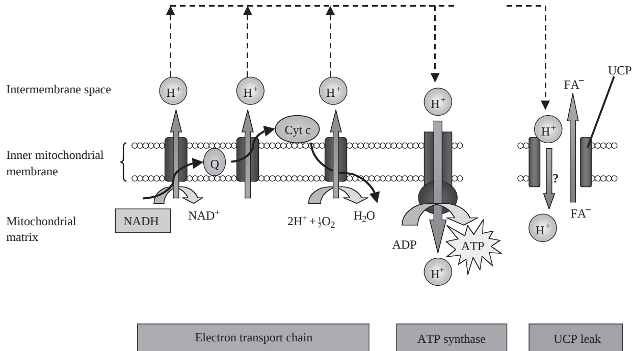
Fig. 1. Action of the electron transport chain leading to the build-up of a proton gradient across the inner mitochondrial membrane. Protons can cross the inner mitochondrial membrane via the F 0 F 1 complex, thereby providing energy for the conversion of ADP to ATP. Alternatively, the proton gradient can be reduced by uncoupling proteins (UCP), either by direct transport of protons from the intermembrane space to the matrix or by transport of fatty acid anions in the opposite direction. Cyt c, cytochrome c. Q, coenzyme Q.
